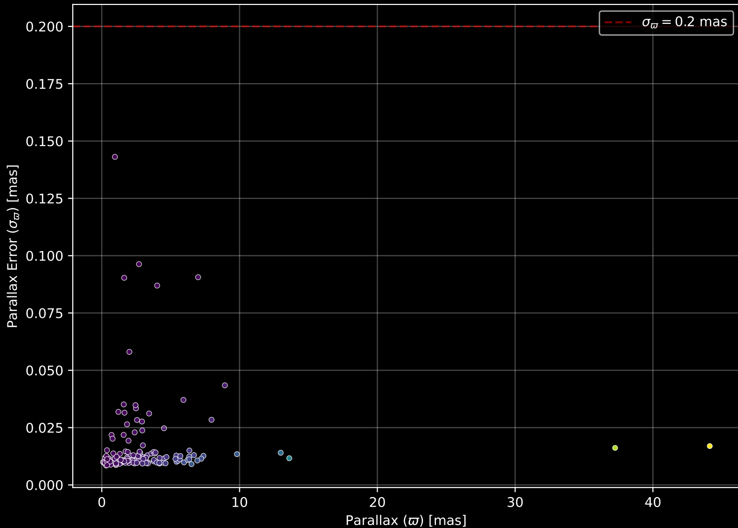
APOGEE DR17 Field: [062+39_MGA] Parallax Quality (n= 149)
