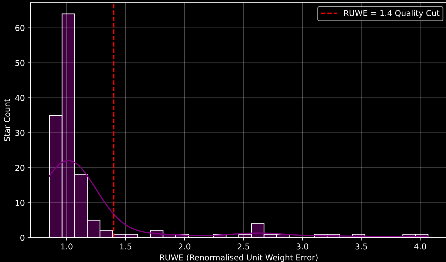
GAPOGEE DR17 Field [062+39_MGA] RUWE Distribution (n= 143)
