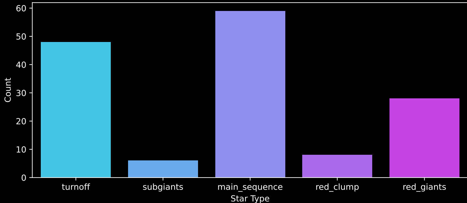
APOGEE DR17 Field: [062+39_MGA] Count plot of Star Type
