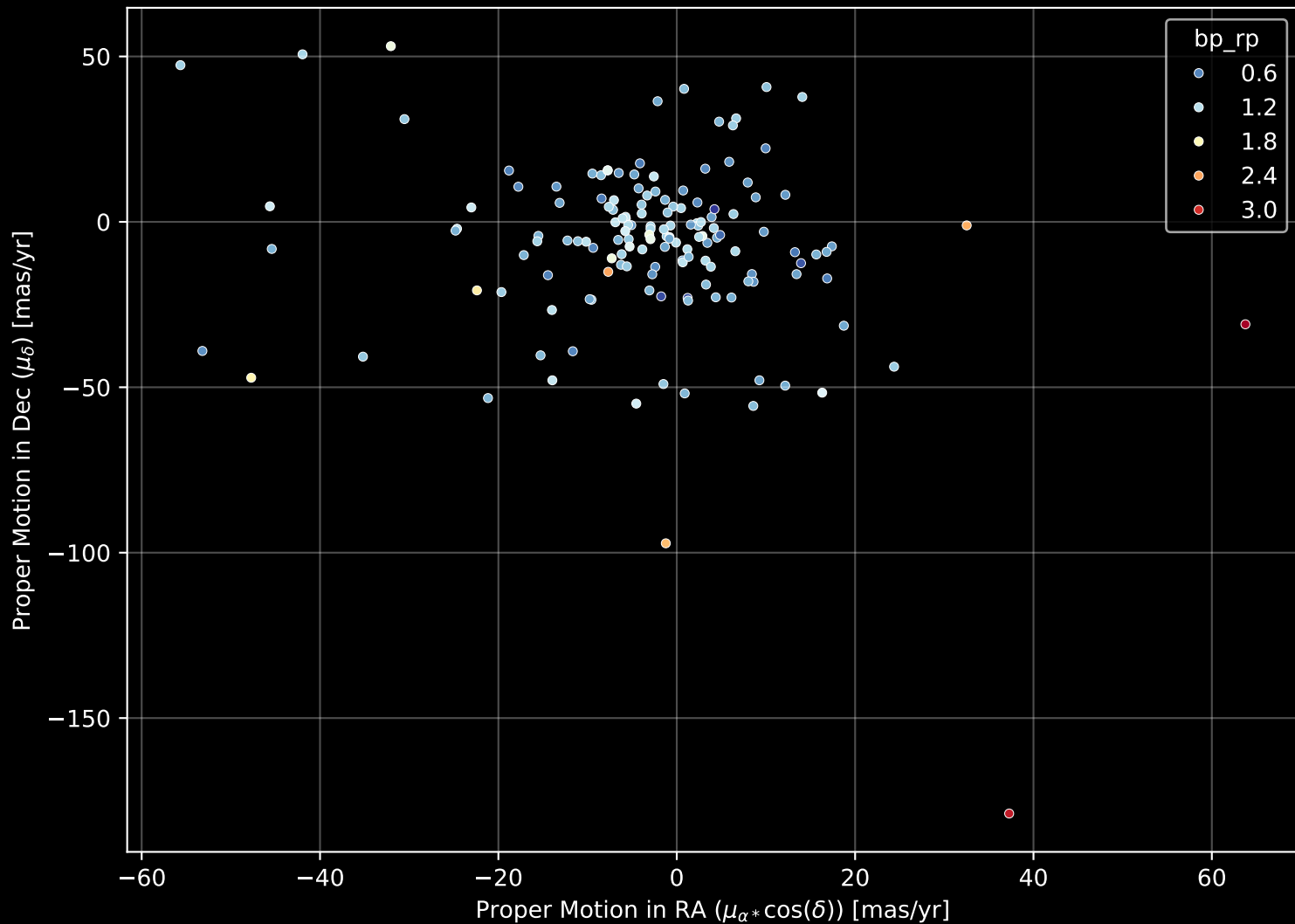
APOGEE DR17 Field: [062+39_MGA] Proper Motion Diagram (n= 149)
