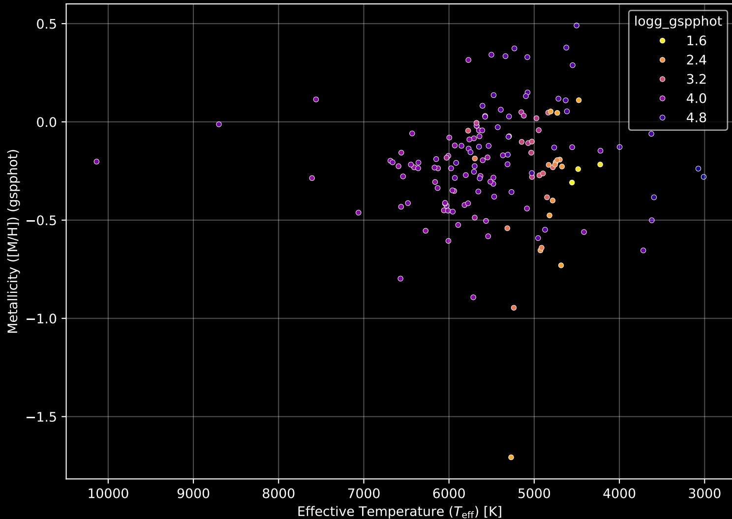
APOGEE DR17 Field: [062+39_MGA] Stellar Population Parameters (n= 149)
